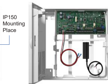
MG5075 with 110-220V / 15 Vdc / 60W Wall Plug
