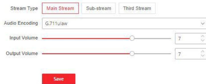
Figure 8-6 Audio Settings
