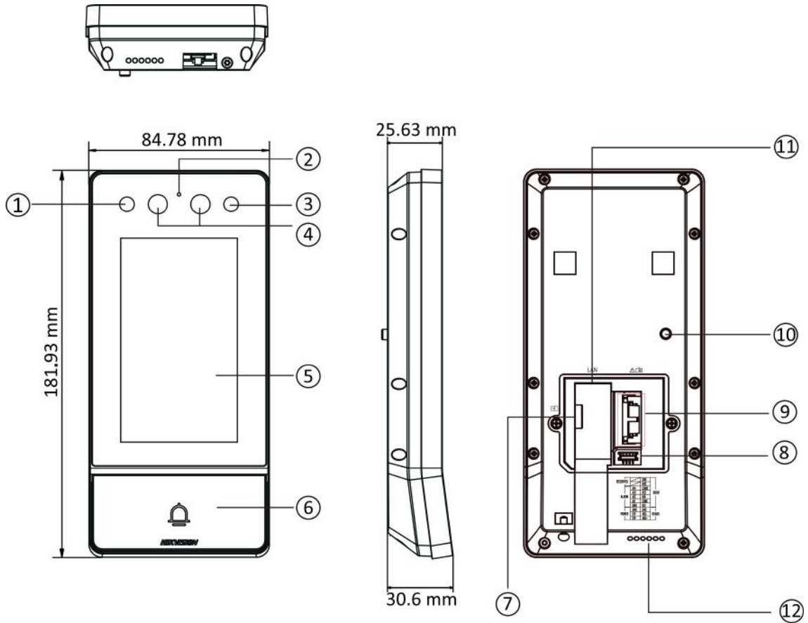
Figure 1-1 Device Appearance
