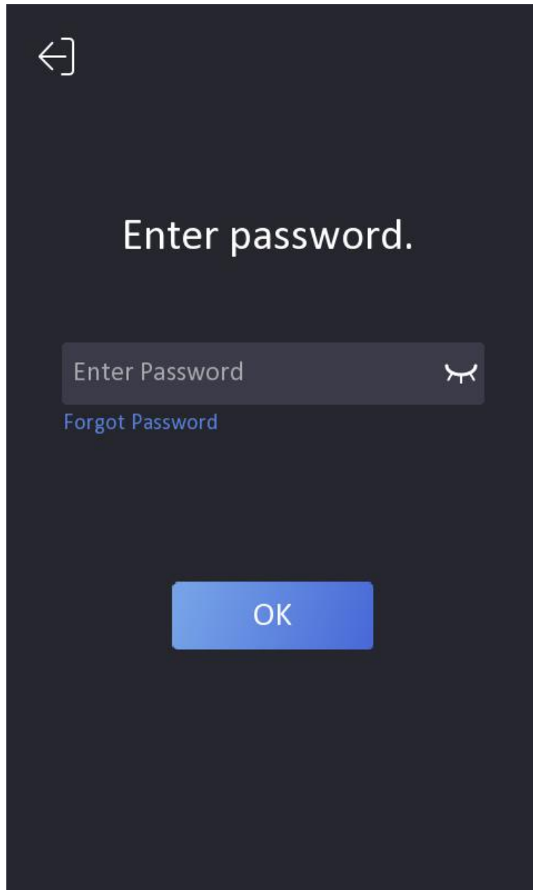
Figure 5-8 Authentication Page
