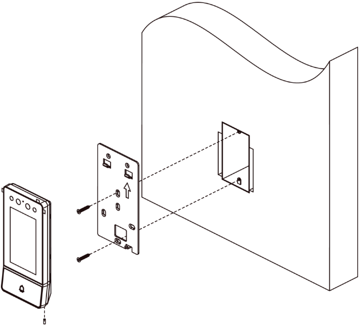
Figure 3-4 Flush Mounting
