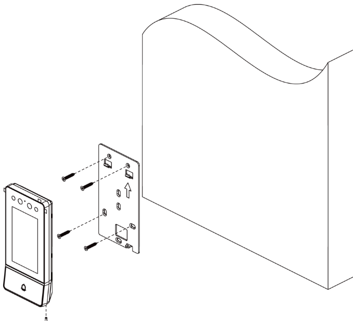
Figure 3-3 Surface Mounting
