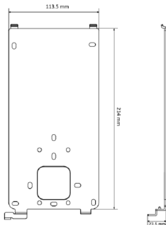
Figure 4-2 Mounting Plate
