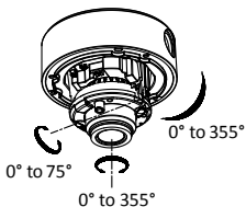
Figure 2. 4 3-Axis Adjustment
