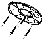
Figure 2. 2 Attach the Back Box/Base Plate
