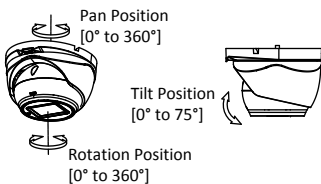
Figure 2-12 3-axis Adjustment
