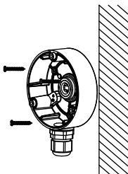
Figure 2-5 Secure the Junction Box on the Wall
