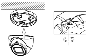
Figure 2-11 Install the Turret Camera
