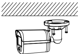
Figure 2-9 Secure Camera to Ceiling
