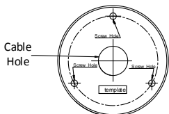
Figure 2-8 Drill Template
