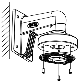
Figure 2-23 Fix Gang Box
