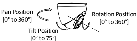
Figure 2-15 3-Axis Adjustment
