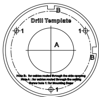
Figure 2-4 Drill Template for Junction Box
