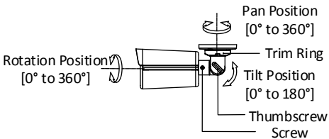
Figure 2-3 3-Axis Adjustment
