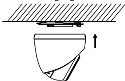
Figure 2-13 Fit Camera
