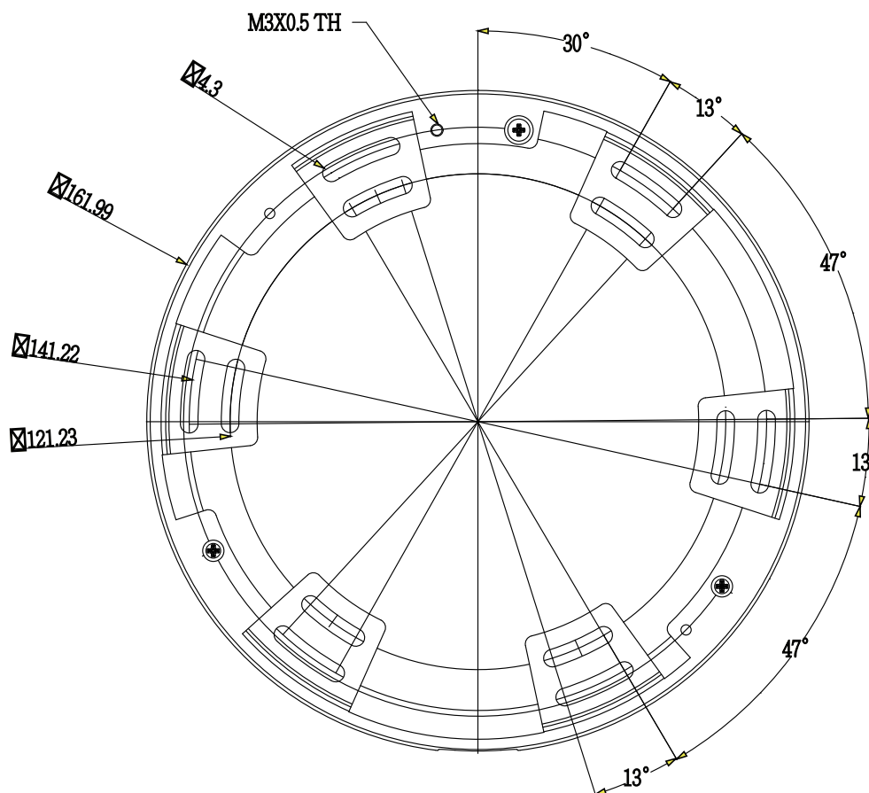
Camera Mounting Plate Mounting Positions
