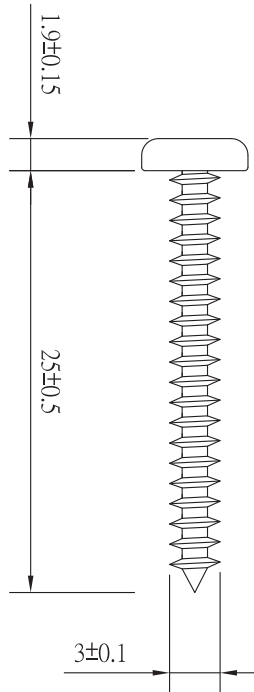
Pan head M3x25 self-tapping
