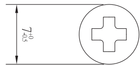
Pan head M4x8
