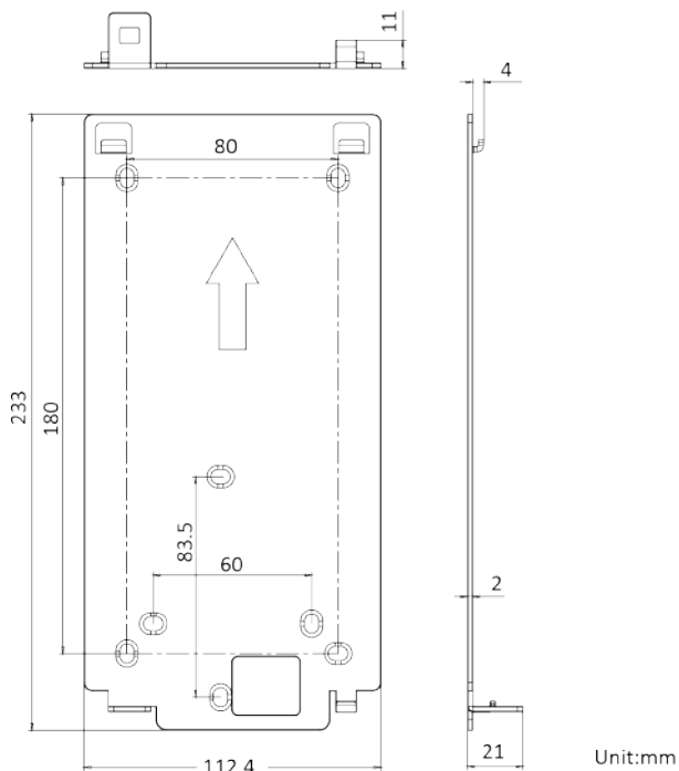
Figure 4-5 Mounting Plate
