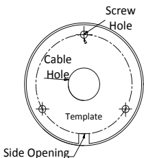
Figure 2-8 Drill Template
