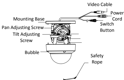
Figure 1-4 Overview of Type III Camera
