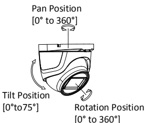
Figure 2-15 3-axis Adjustment
