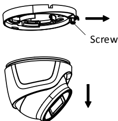
Figure 2-11 Disassemble the Camera
