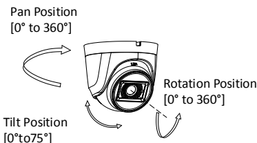
Figure 2-10 3-axis Adjustment
