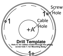
Figure 2-16 Drill Template
