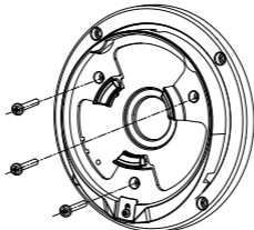
Figure 2-14 Secure Screws on Junction Box's Cover
