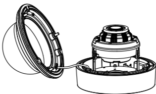
Figure 2-16 Remove the Bubble
