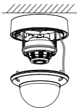
Figure 2-19 Install the Bubble Back
