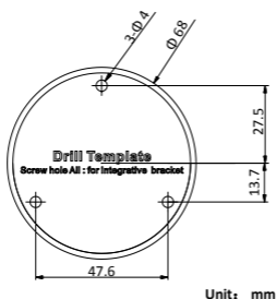
Figure 2. 1 Drill Template
