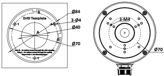
Figure 2-5 Drill Template
