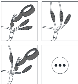
Figure 2-10 Waterproof Cables
