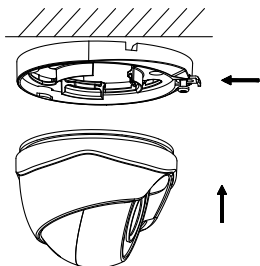
Figure 2-3 Secure the Camera
