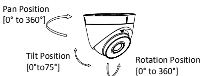
Figure 2-11 3-Axis Adjustment
