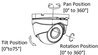
Figure 2-4 3-Axis Adjustment
