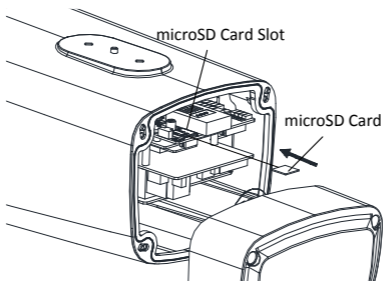
Figure 2-3 Insert micro SD Card
