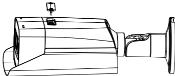
Figure 2-5 Remove Card Slot Cover
