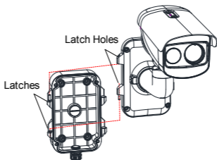
Figure 2-19 Take Apart Junction Box
