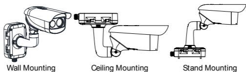
Figure 2-18 Type III Camera Installation Methods
