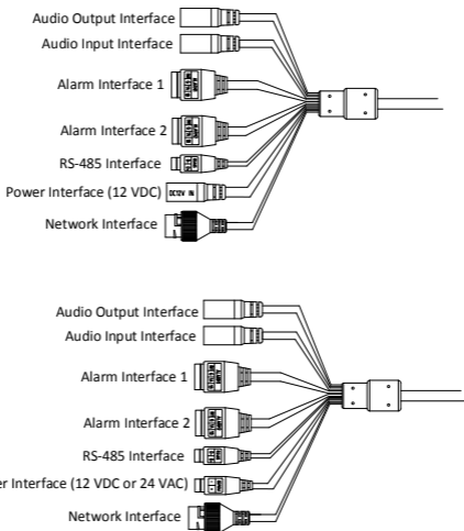
Figure 1-8 Cable Description
