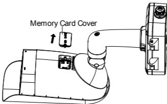
Figure 2-7 Remove Card Slot Cover
