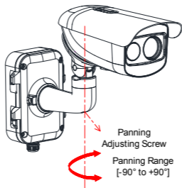
Figure 2-25 P-Axis Adjustment
