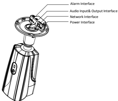
Figure 1-9 Interface Description
