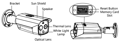
Figure 1-7 Type IV Camera Appearance
