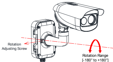
Figure 2-23 R-Axis Adjustment
