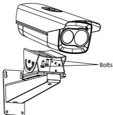
Figure 2-10 Fix the Camera to the Bracket
