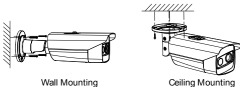
Figure 2-15 Wall/Ceiling Mounting
