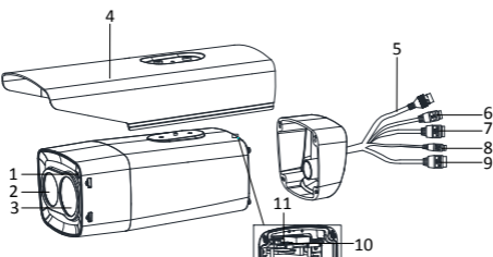
Figure 1-1 Type I Camera Appearance (1)
