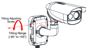
Figure 2-24 T-Axis Adjustment
