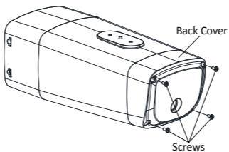
Figure 2-2 Remove Back Cover Case
