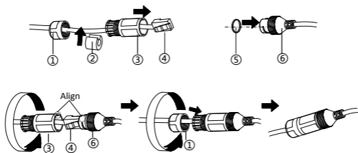
Figure 2-26 Install Waterproof Jacket
