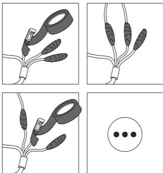
Figure 2-27 Waterproof Cables
