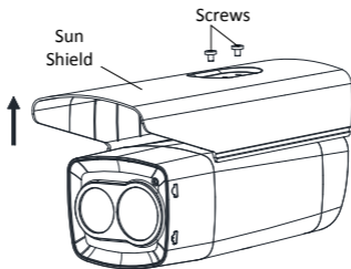
Figure 2-1 Remove Sun Shield
