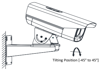
Figure 2-13 Tilt Adjustment
