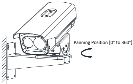
Figure 2-12 Pan Adjustment
