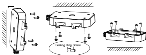
Figure 2-21 Install Junction Box Base
