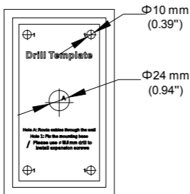
Figure 2-20 Drill Template
