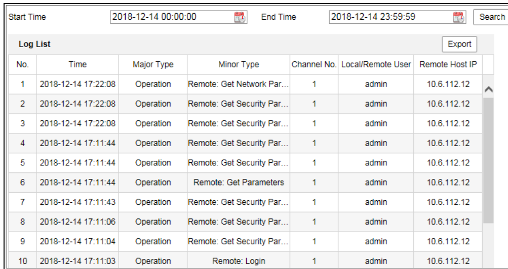
Figure 6-11 Log Searching
