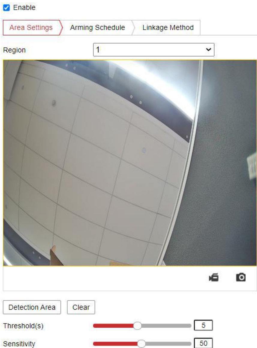
Figure 8-17 Loitering Detection
