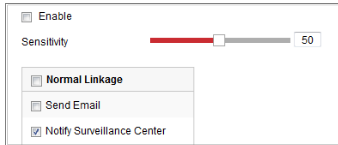
Figure 8-8 Defocus Detection
