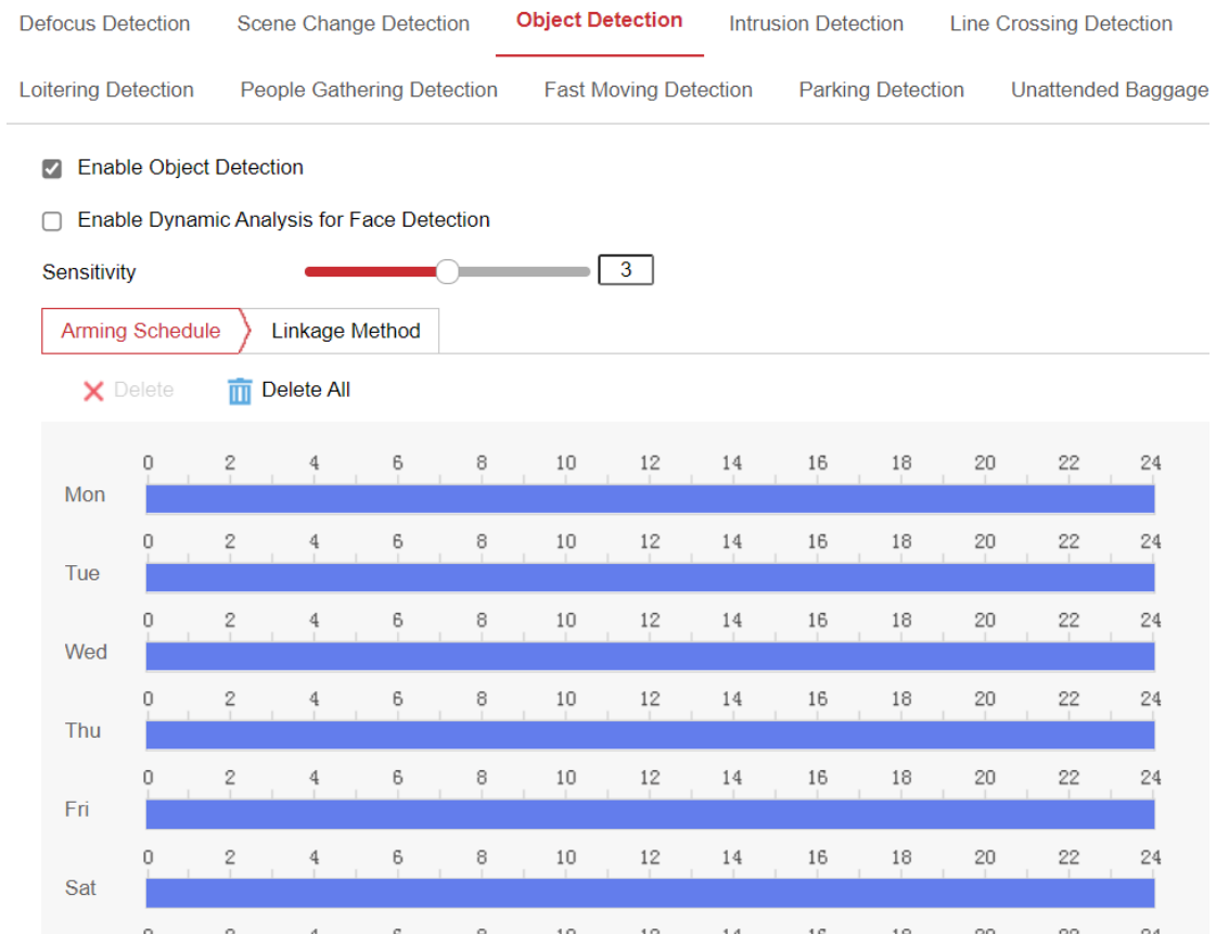
Figure 8-10 Object Detection
