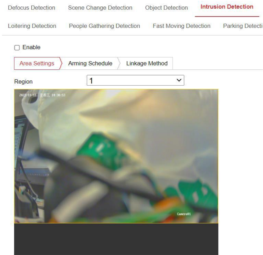
Figure 8-11 Intrusion Detection
