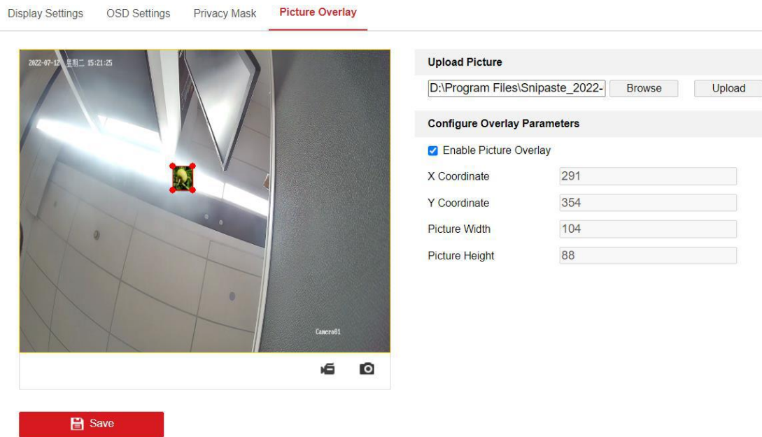
Figure 7-8 Picture Overlay
