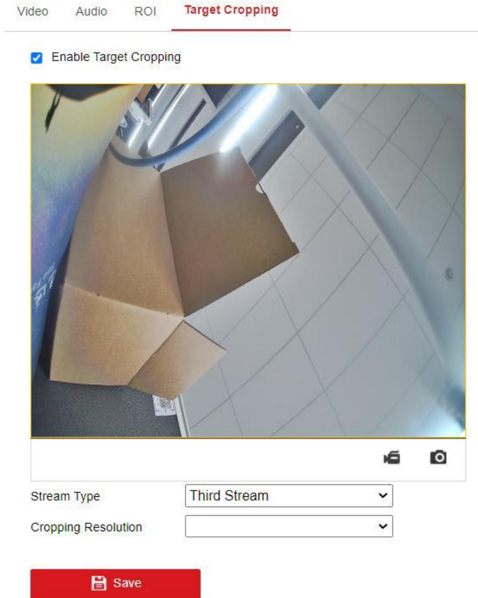
Figure 6-4 Target Cropping
