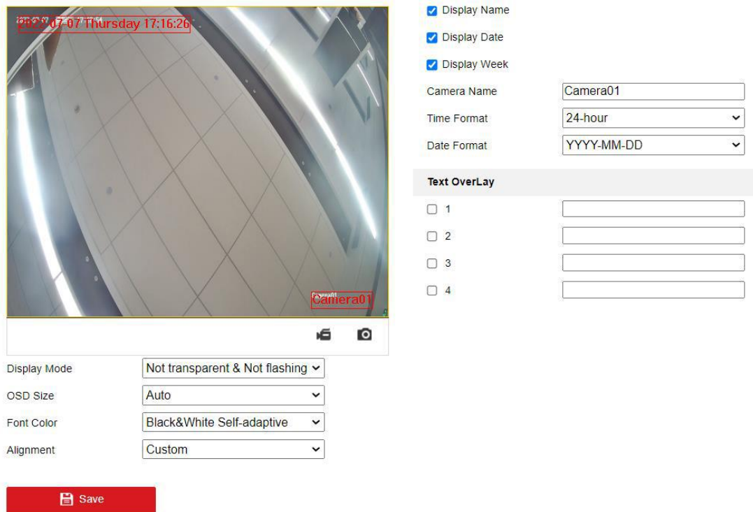
Figure 7-6 OSD Settings
